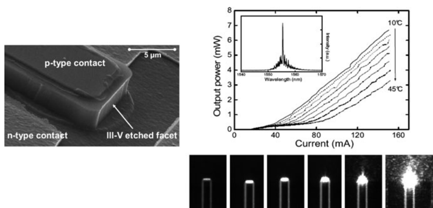
Fig. 9.24 SEM picture of an InGaAsP/InP laser on silicon with ICP \text{Cl}_2/\text{H}_2 etched facets, L-I curves obtained at different temperatures with a spectrum in the inset obtained at 15 °C, and infrared images of the FP laser obtained at different currents
