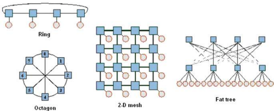
Fig. 6.4 Different NoC topologies
