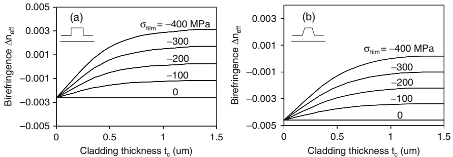
Fig. 2.10 Total modal birefringence \Delta n_{\text{eff}} as a function of the oxide upper cladding thickness t_c , for different cladding stress levels \sigma_{\text{film}} of 0, -100, -200, -300, and -400 MPa, respectively. (a) The vertical sidewall waveguide as shown in Fig. 2.7; (b) the trapezoidal waveguide as shown in Fig. 2.8
