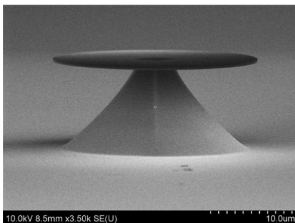
Fig. 4.24 SEM image of a fabricated SRSN:Er microdisk. The pedestal is 11\text{ }\mu\text{m} high, with a center contact patch diameter of 5.2\text{ }\mu\text{m}
