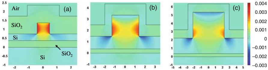
Fig. 2.14 Material birefringence ( n_y - n_x ) in SOI waveguides with a width of 0.9 H , and an aspect ratio r of 0.375 , for ridge height H of (a) 1 \mu\text{m} , (b) 3 \mu\text{m} , and (c) 5 \mu\text{m} . The oxide thickness is 1 \mu\text{m} , with a stress \sigma_{\text{film}} = -105 \text{ MPa}
