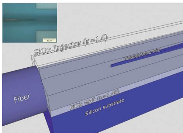
Fig. 9.11 3D representation of the fiber coupler. Insert: Nomarsky image of the silicon nano-tip
