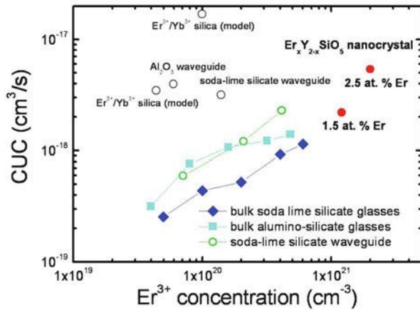
Fig. 4.22 Reported values of the cooperative upconversion coefficient at the ^4\text{I}_{13/2} energy level of Er in various hosts from [73]. For comparison, the cooperative upconversion coefficients obtained for \text{Er}_x\text{Y}_{2-x}\text{SiO}_5 with 1.5 and 2.5 at.% Er are indicated by filled circles
