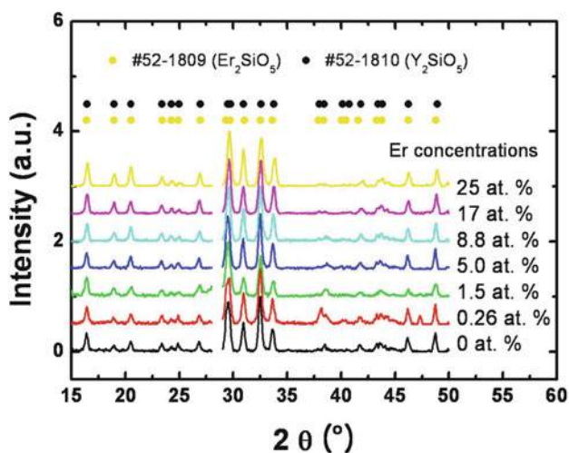
Fig. 4.17 The fixed \theta X-ray diffraction (XRD) spectra from nanocrystals fabricated with various \text{Er} concentrations. Also shown are the expected XRD peak positions of \text{Er}_2\text{SiO}_5 and \text{Y}_2\text{SiO}_5
