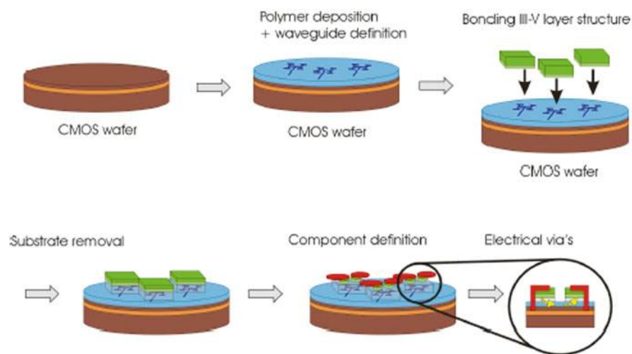
Fig. 6.11 Above-IC approach
