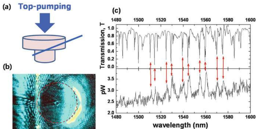
Fig. 4.32 (a) A schematic description and (b) a CCD image of an SRSN:Er microdisk under top pumping. The position of the disk is indicated by the dotted circle . A 473-nm DPSS laser was used to illuminate the edge of the disk, and a tapered fiber was used to measure both the transmission and emission spectra shown on the right. Note the exact correspondence between the dips in transmission and the peaks in emission. The width of the emission peaks is limited by the detector resolution, which was set at 2 nm
