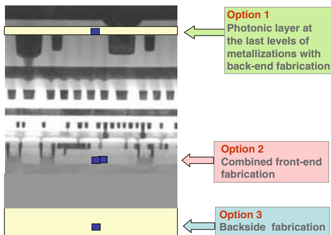
Fig. 9.1 Integration routes
