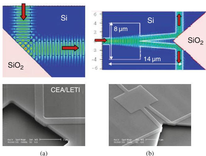
Fig. 9.6 3D-finite-difference time-domain (FDTD) simulations and scanning electron microscope views of (a) a corner mirror and (b) a compact T-splitter based on rib waveguides
