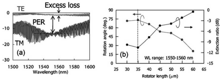
Fig. 1.31 (a) Measured transmission spectra of the polarization rotator with a length of 35\text{ }\mu\text{m} ; (b) Polarization rotation angle estimated by the measured Poincare map and polarization extinction ratio calculated from the measured rotation angle
