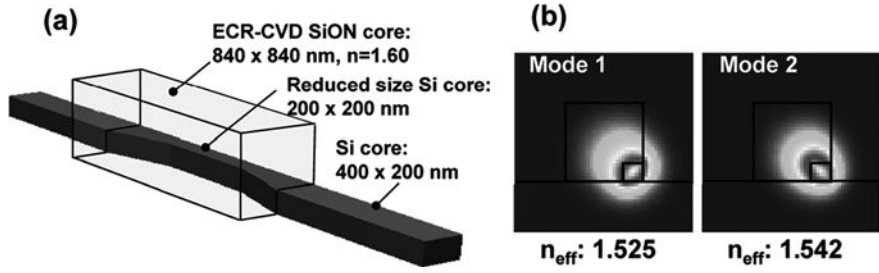
Fig. 1.30 (a) Schematic of the polarization rotation structure and (b) its eigenmodes
